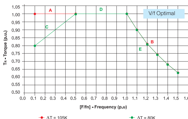
Figure 33 – Derating curve for optimal flux®
