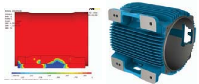
Figure 4 – Solid feet
