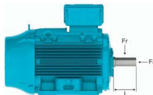
Figure 25 – Radial and axial thrust on motor shaft
